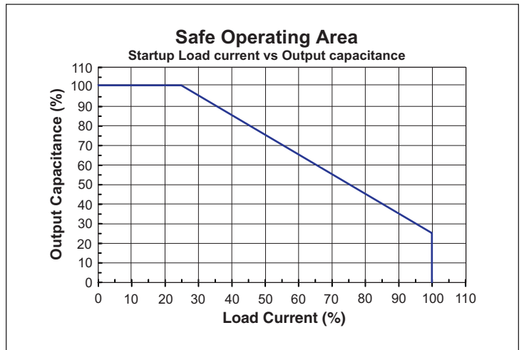
Figure 13 — Start up load current vs. output capacitance
