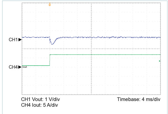
Figure 6 — 10% to 100% load transient response, V_{IN} = 28\text{ V} , nominal trim, C_{OUT\_EXT} = 200\ \mu\text{F}
