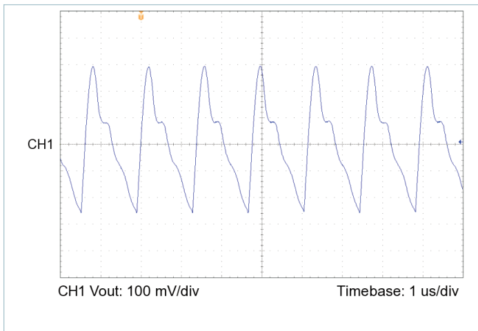
Figure 17 — Output voltage ripple, V_{IN} = 28\text{ V} , V_{OUT} = 48.0\text{ V} , C_{OUT\_EXT} = 200\ \mu\text{F} , R_{LOAD} = 7.200\ \Omega
