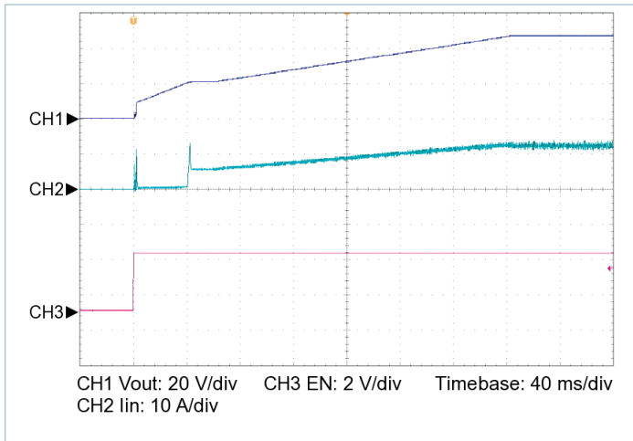
Figure 15 — Startup from EN, V_{IN} = 28\text{ V} , C_{OUT\_EXT} = 2000\ \mu\text{F} , R_{LOAD} = 7.200\ \Omega
