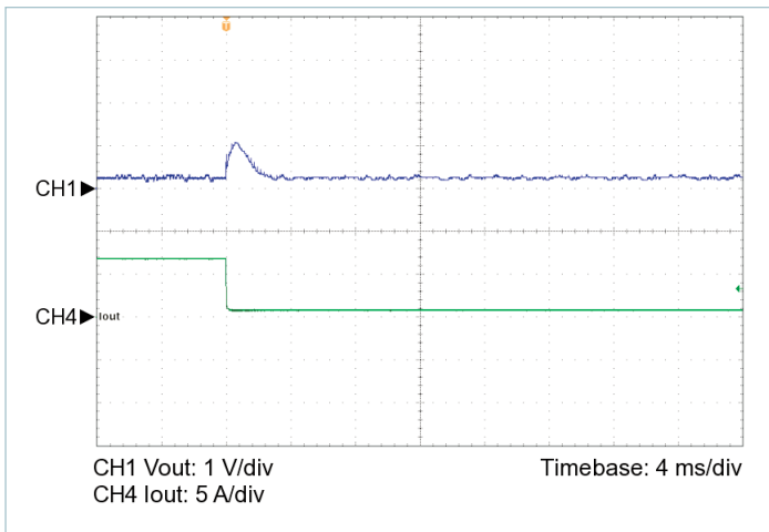
Figure 5 — 100% to 10% load transient response, V_{IN} = 28\text{ V} , nominal trim, C_{OUT\_EXT} = 200\ \mu\text{F}
