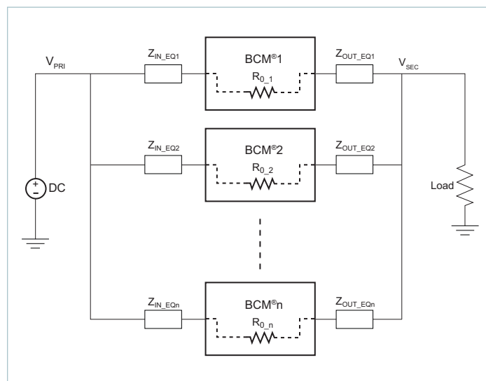
Figure 19 — BCM parallel array
