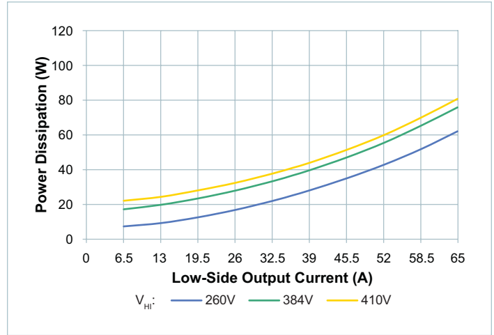
Figure 4 — Power dissipation at T_{TOP}, T_{BOTTOM} = -40^{\circ}C
