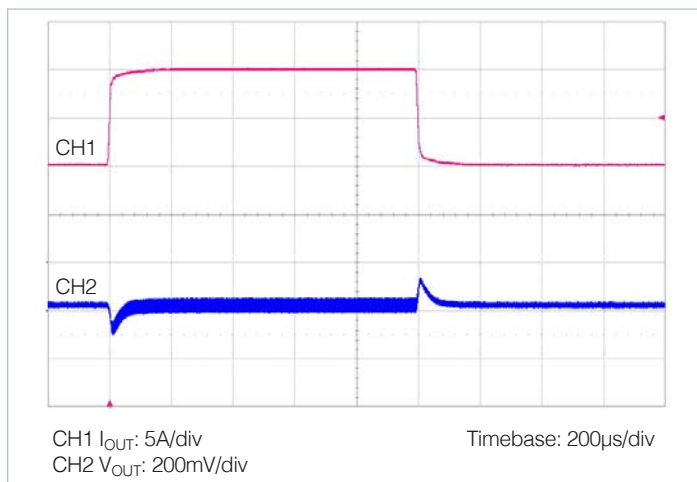
Figure 47 — Transient response: 50 – 100% load, at 1A/μs. nominal line, nominal trim, C OUT = 12 x 47μF ceramic
