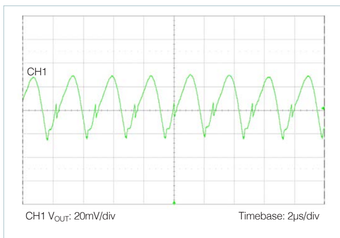
Figure 48 — Output voltage ripple: nominal line, nominal trim, 100% load, C OUT = 12 x 47μF ceramic
