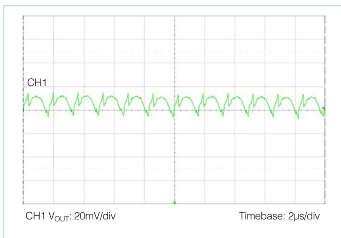
Figure 51 — Output voltage ripple: nominal line, nominal trim, 50% load, C OUT = 12 x 47μF ceramic
