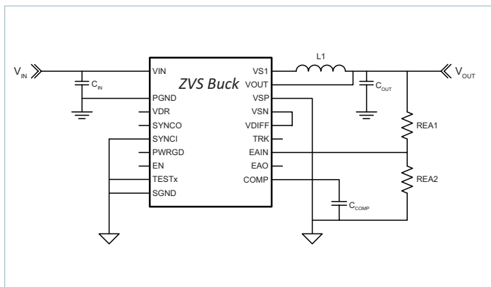
Figure 58 — ZVS Buck with required components
